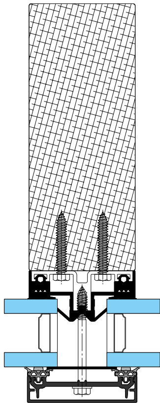
Structure bois*
